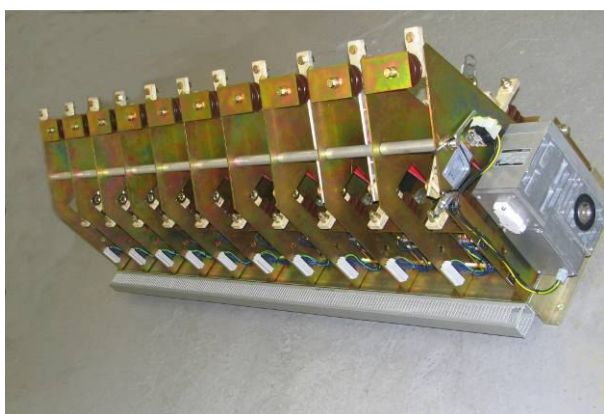
MOD-UI-CI 12kV 630A 10p Modular inverter with motordrive and each pole individually selectable
